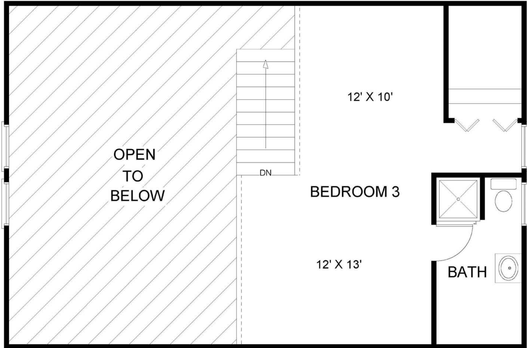
Loft ~ 24' x 20' Plan (9A)
