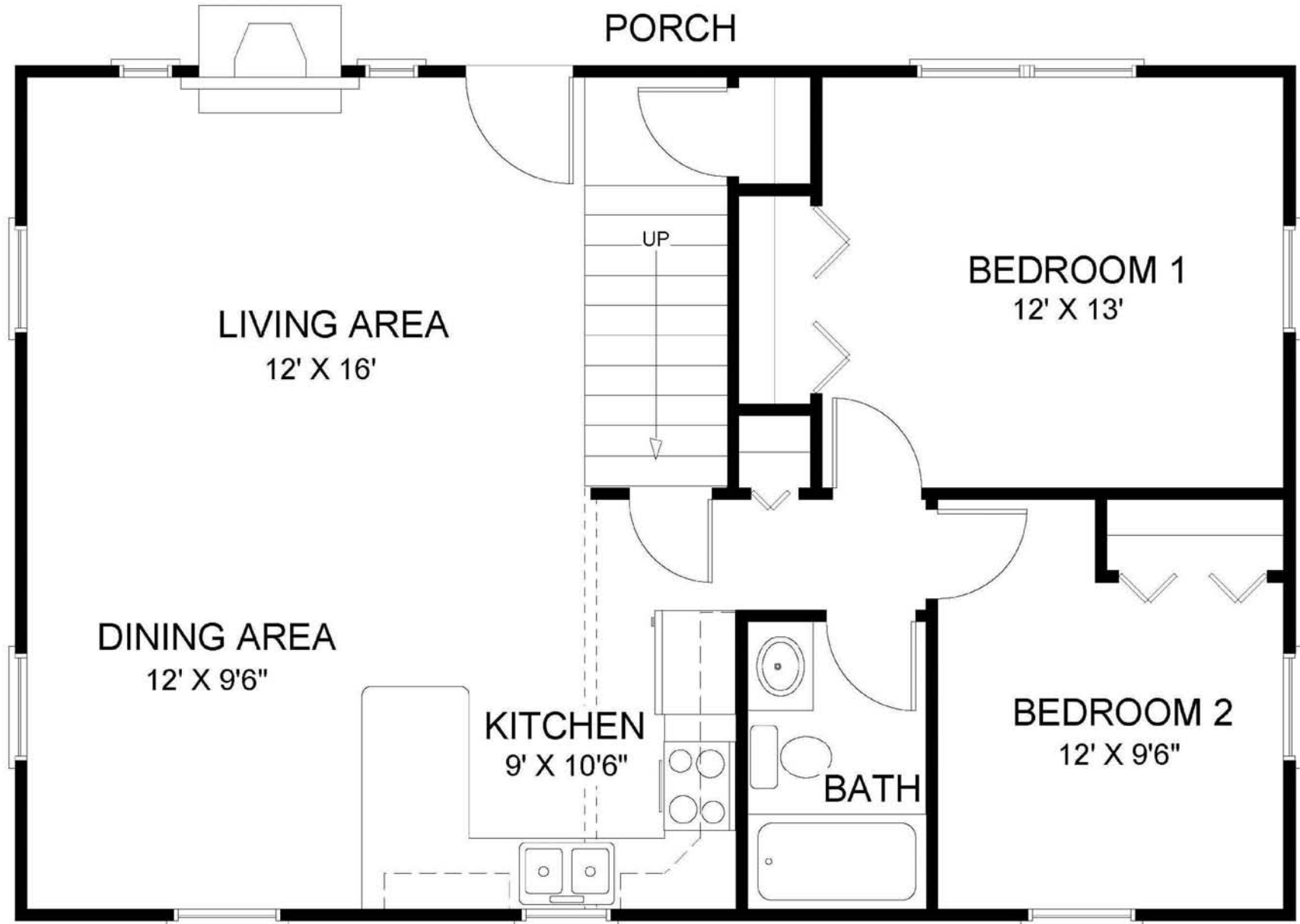
Main Floor ~ 24' x 36' Plan(9)
