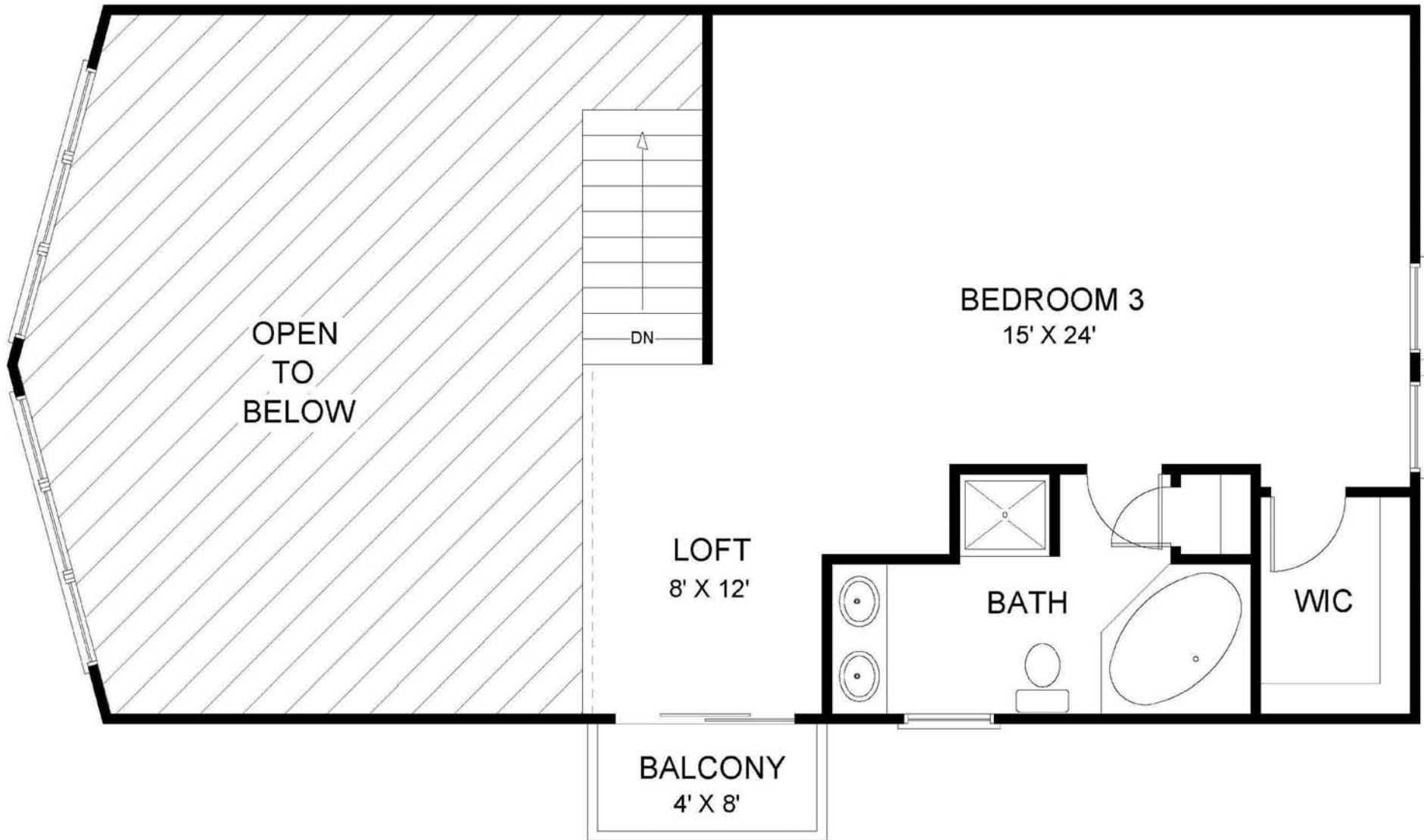
Loft ~ 24' x 28' With Dormer ~ Plan(7A)
