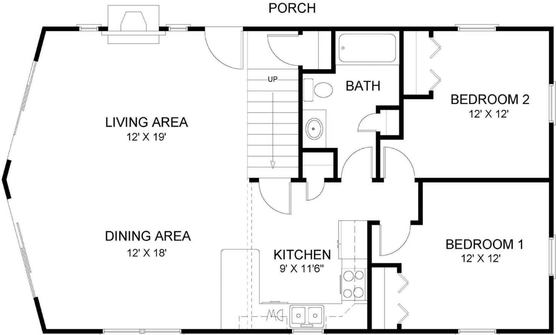
Main Floor ~ 24' x 44' Plan(5)
