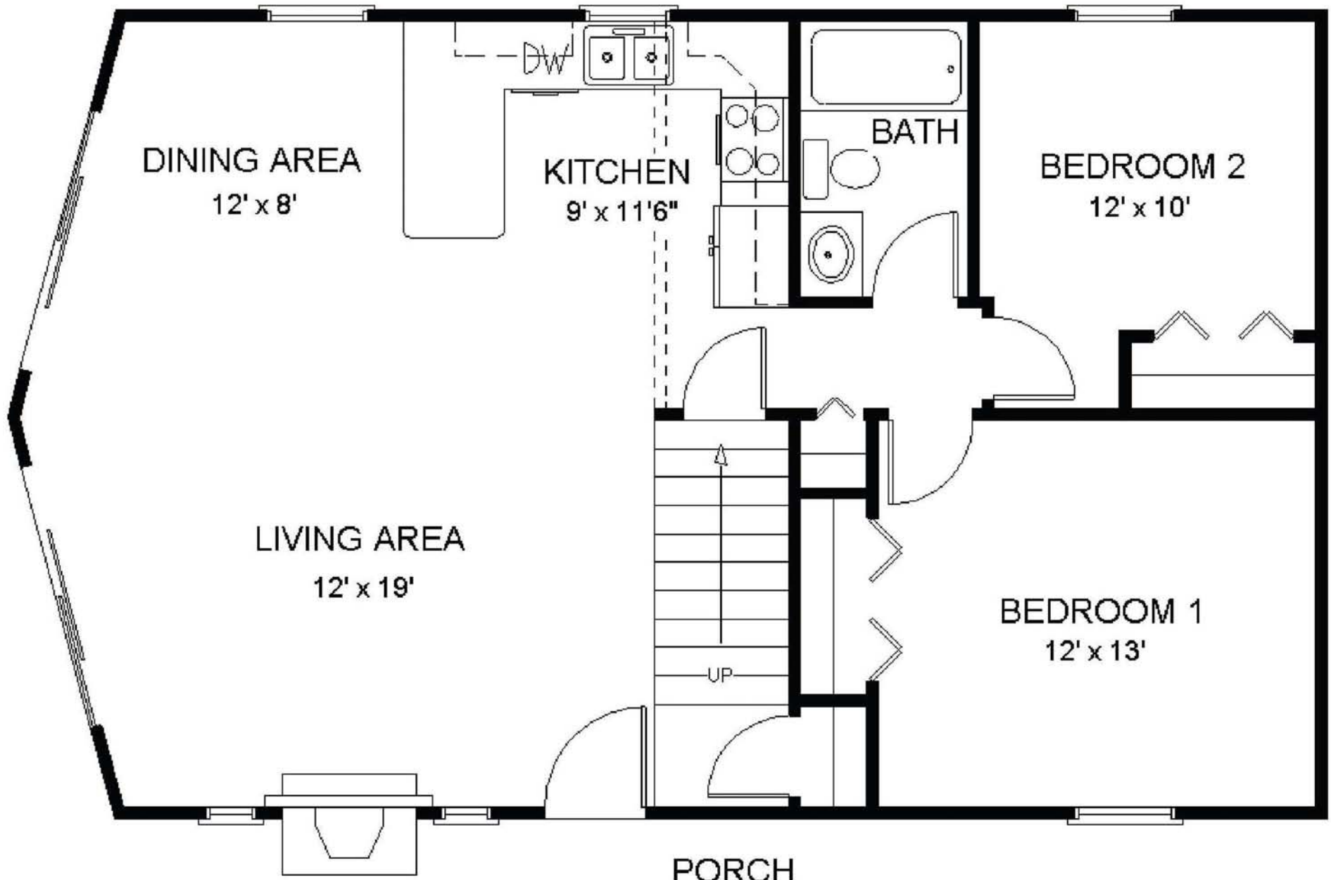
Main Floor ~ 24' x 40' Plan(3)
