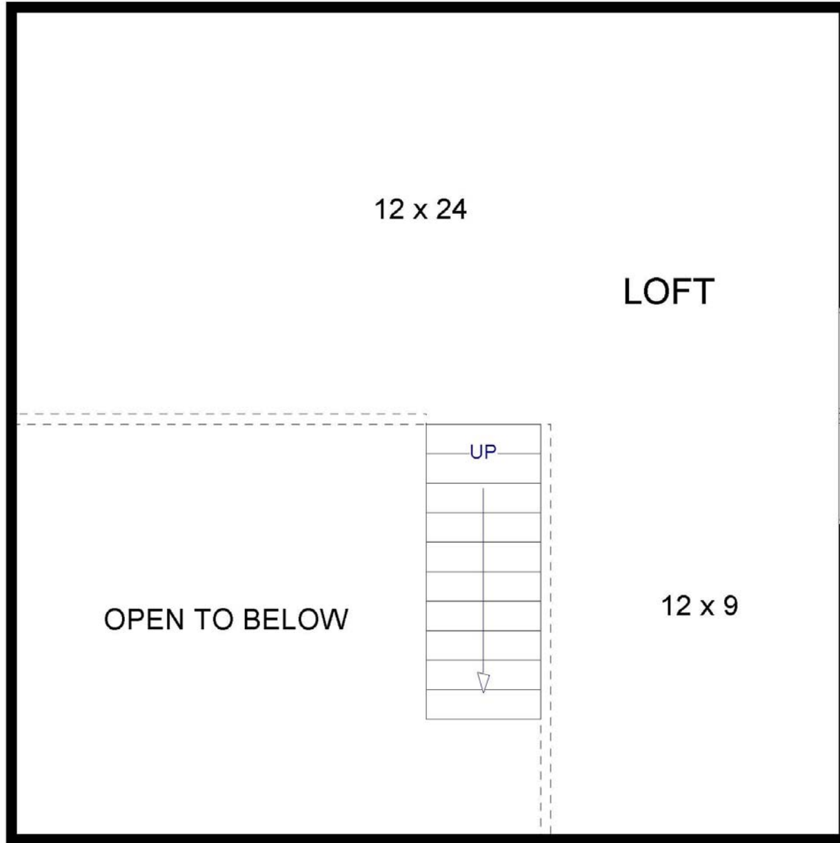
Loft Floor ~ 24' x 24' Plan (22A)
