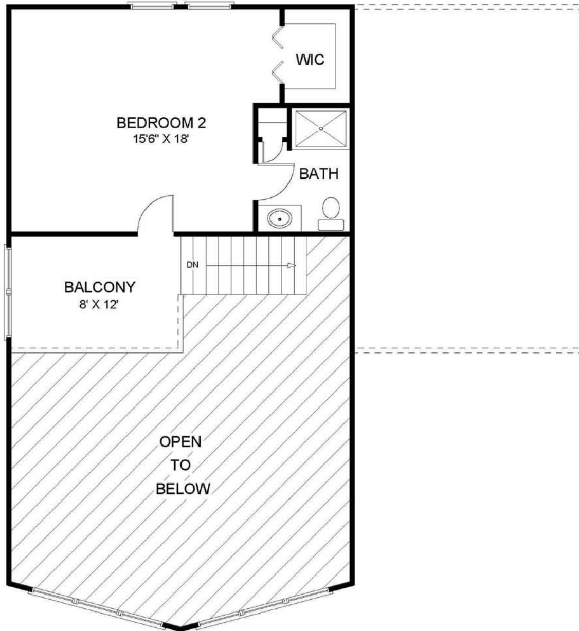
Loft ~ With Dormers ~ Plan (20A)
