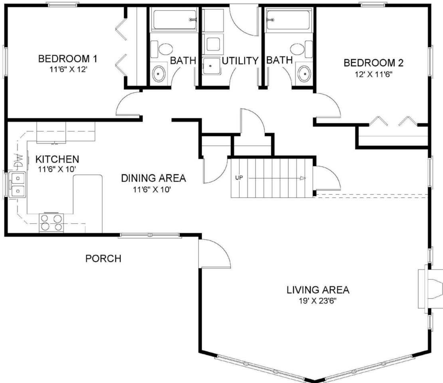
Main Floor ~ Plan (19)
