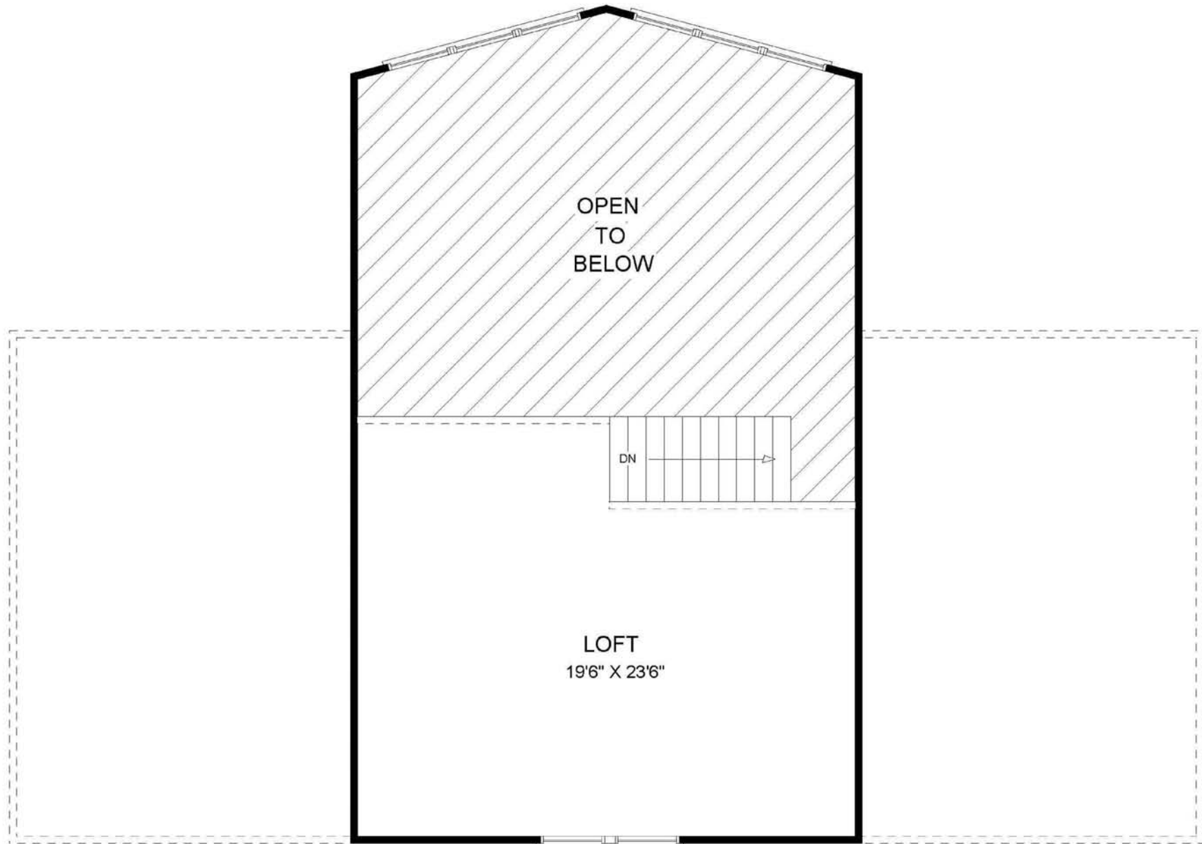
Loft ~24' x 20' Plan (17A)
