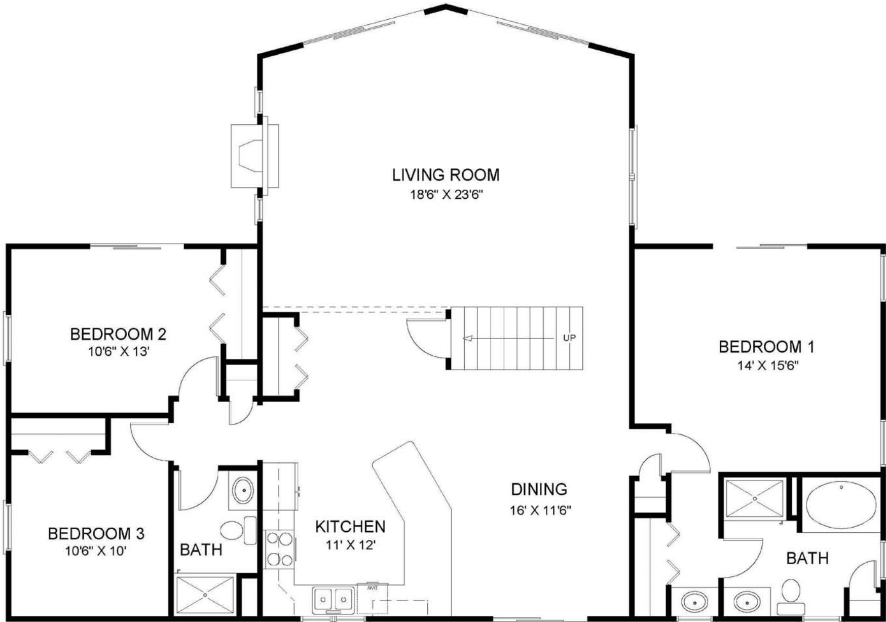
Main Floor ~56' x 36' Plan (17)
