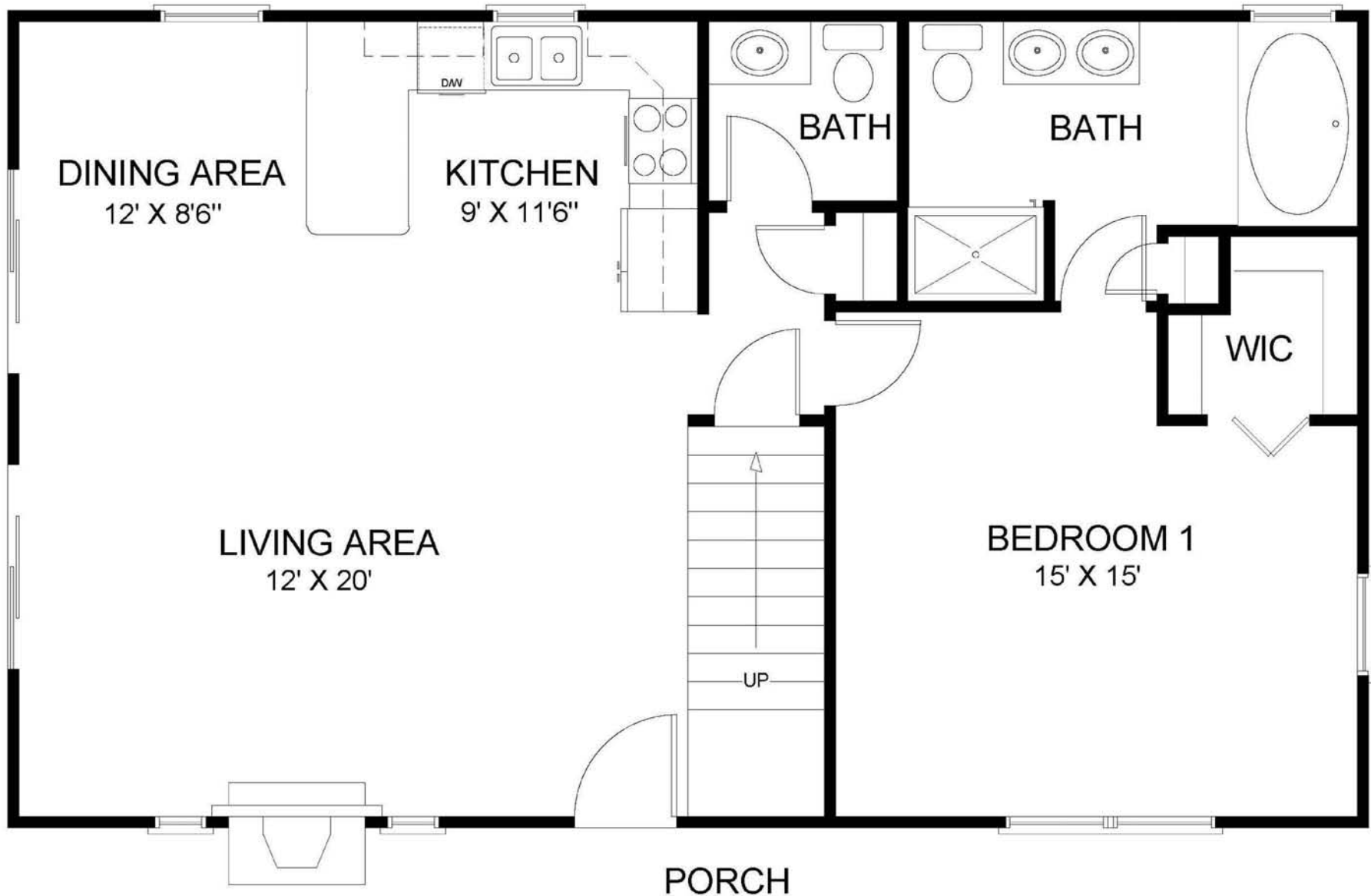
Main Floor ~ 24' x 40' Plan(12)
