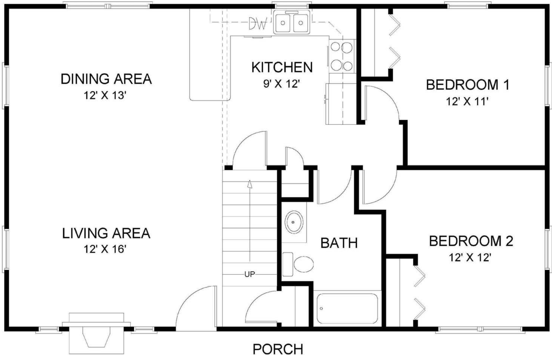
Main Floor ~ 24' x 40' Plan(11)
