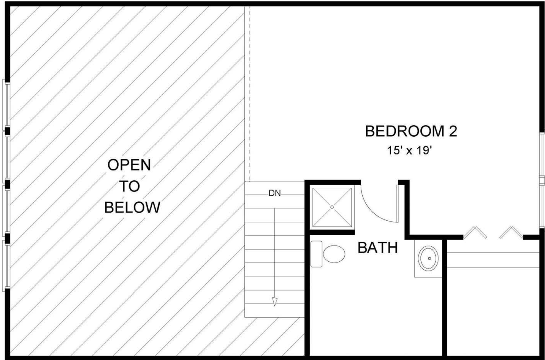
Loft ~ 24' x 20' Plan (10A)
