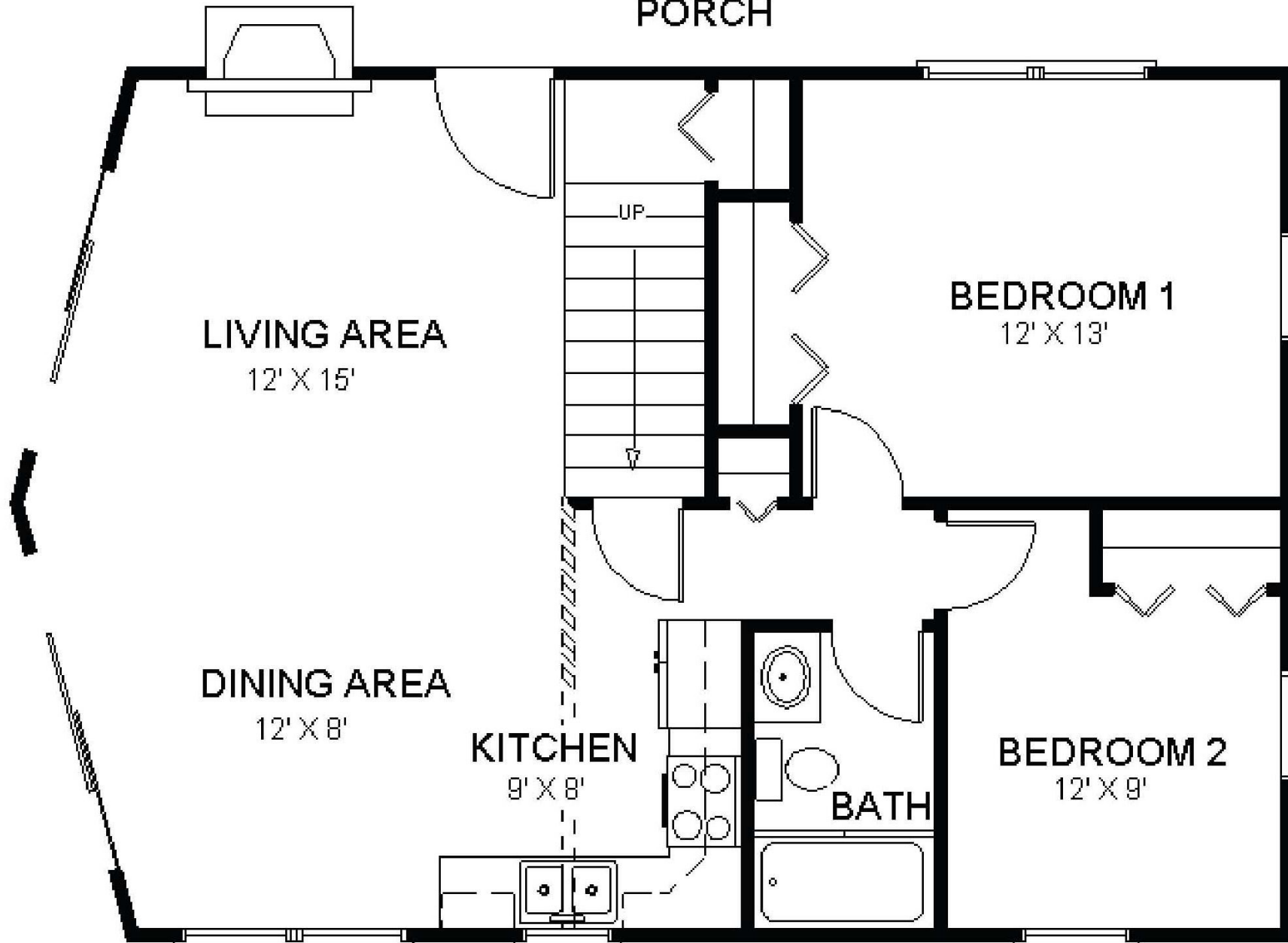
Main Floor ~ 24' x 36' Plan(1)
